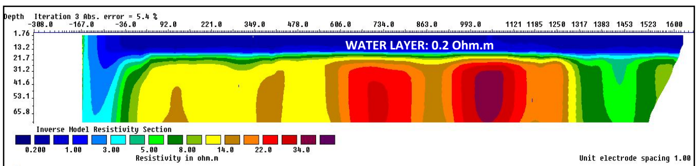
Inversed Resistivity section (5000 data points acquired in 15 minutes)
